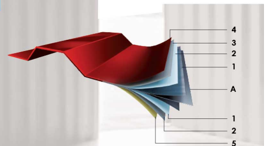
Fundamental Product Structure for Colour-Coated Galvalume
